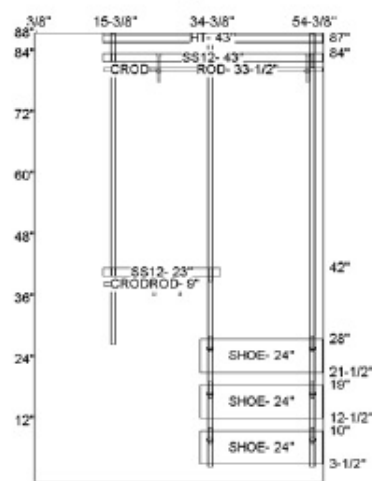
Wall Elevation B
